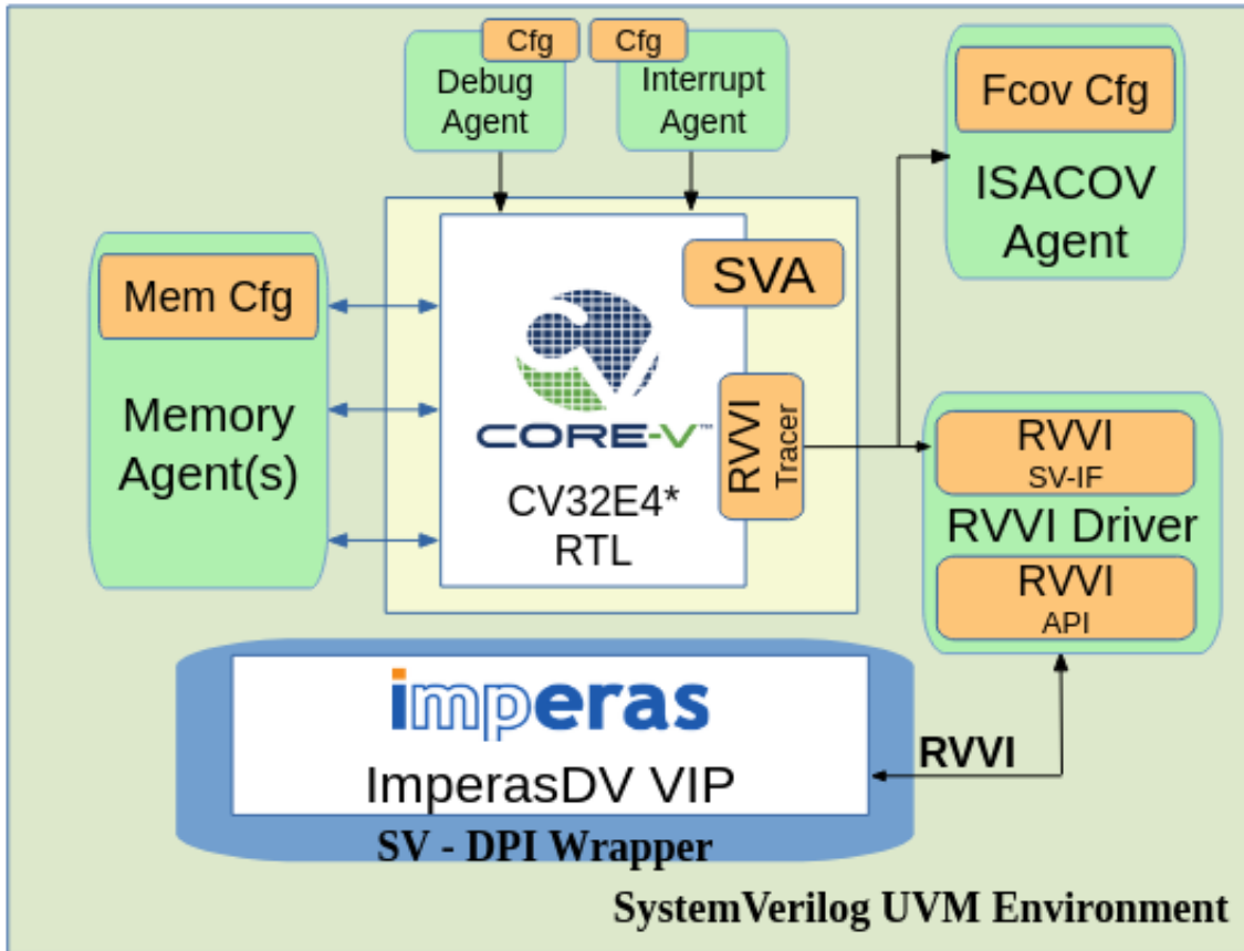
Figure 5: The third generation CORE-V-VERIF environment
