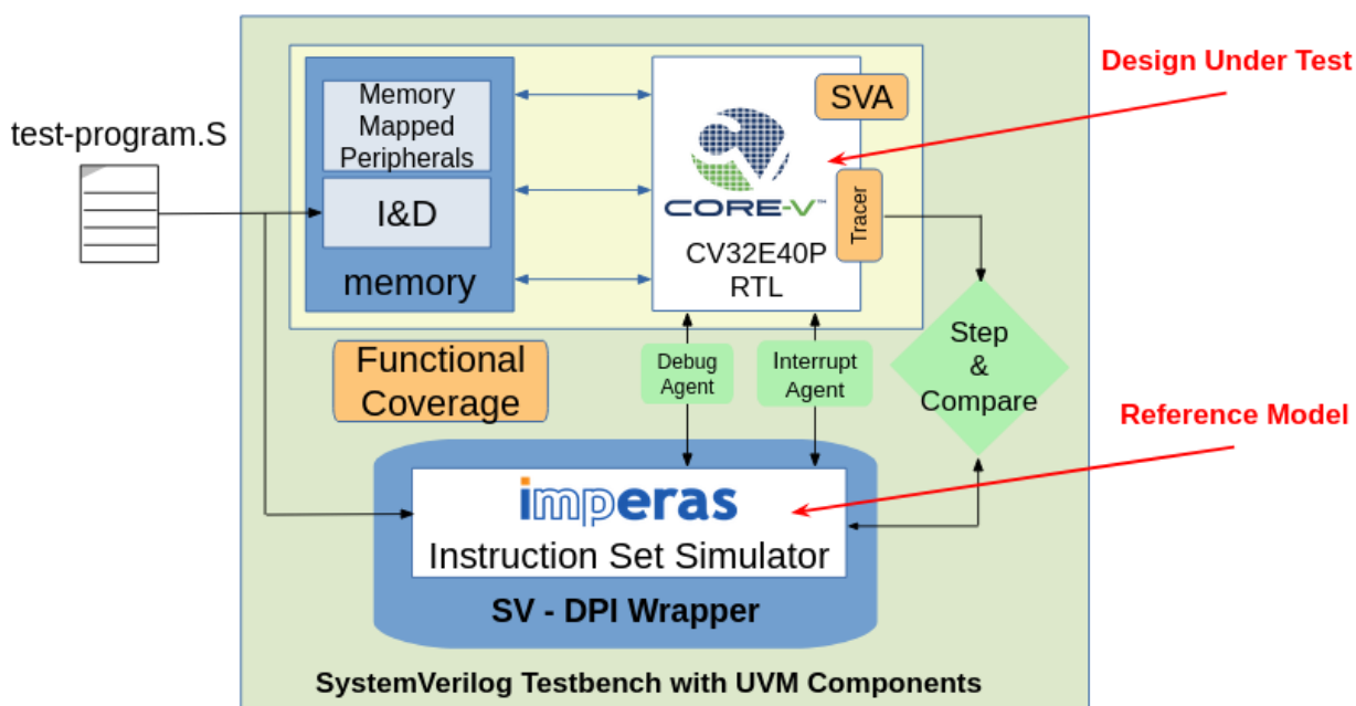
Figure 1: First Generation CORE-V-VERIF environment
