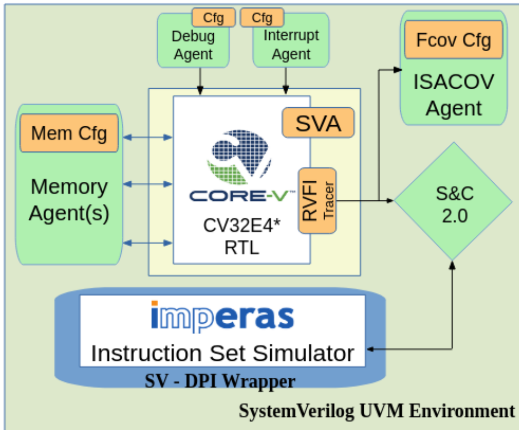
Figure 2: Second Generation CORE-V-VERIF UVM Environment
